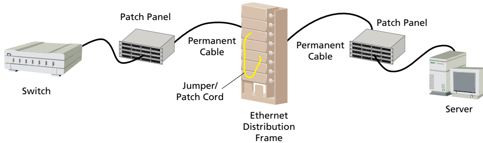
Cross-Connect Diagram
