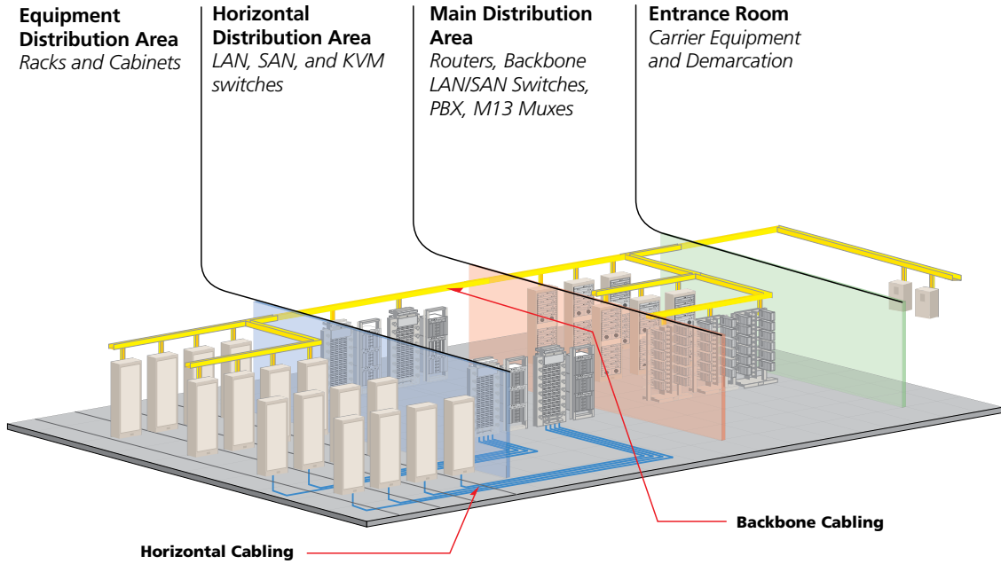
Data Center according to TIA-942
